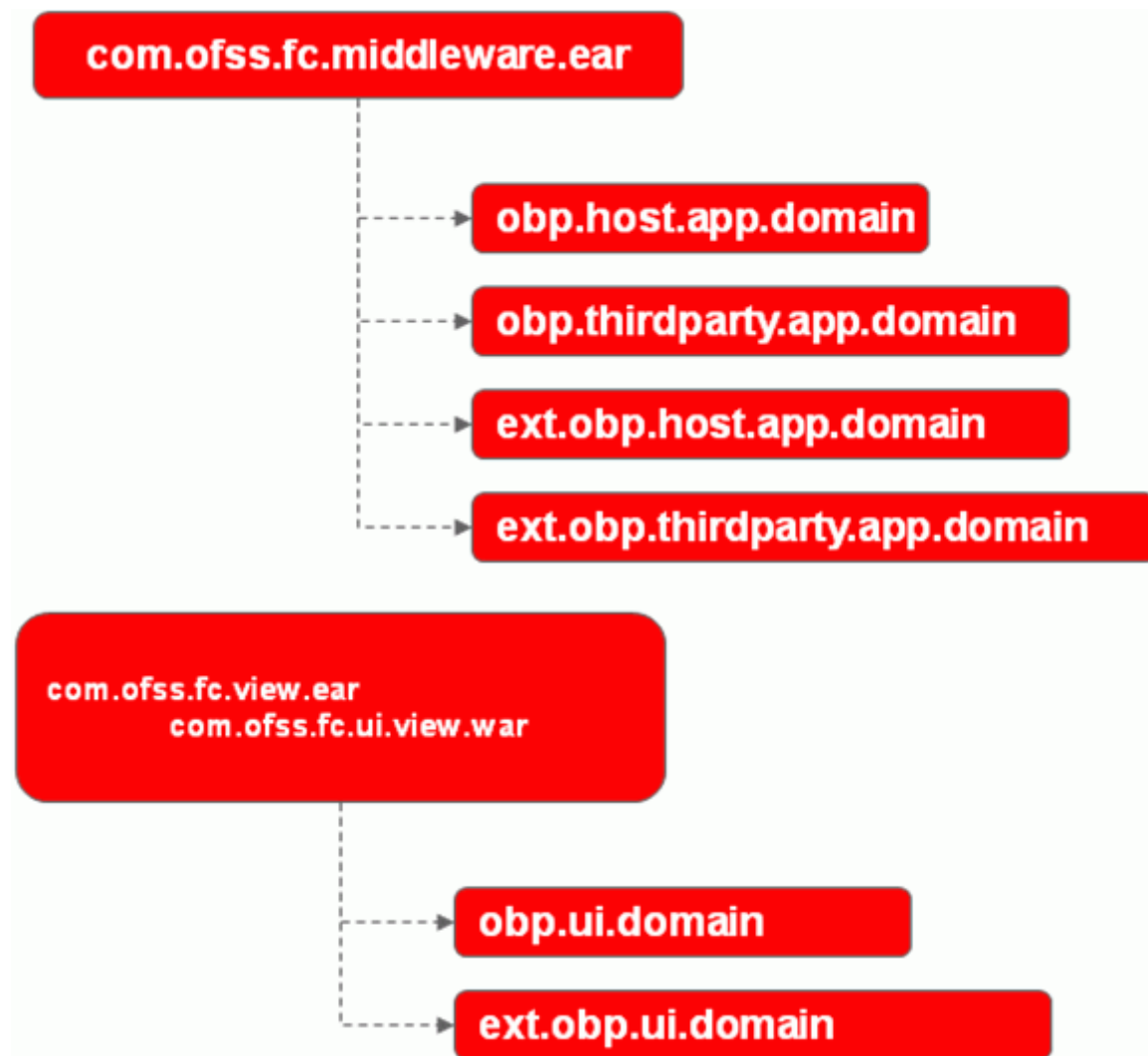
Figure 8–1 Extensibility Deployment
